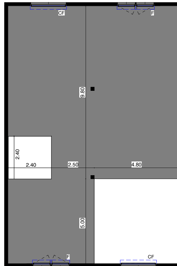
PLAN R+1
