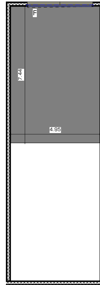
PLAN MEZZANINE
