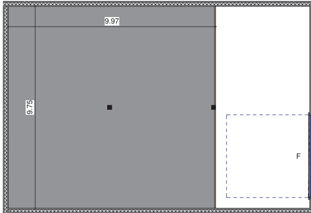
PLAN MEZZANINE
