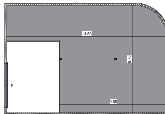
PLAN MEZZANINE
